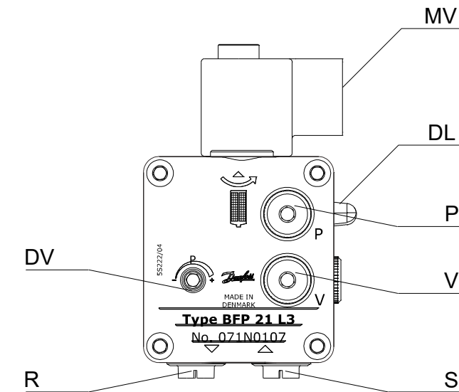
Abb. 14: Danfoss Ölpumpe BFP 21 L3 (7-15 bar)
